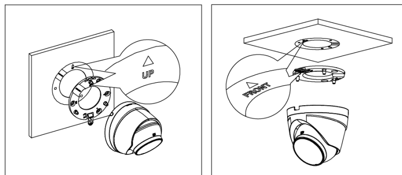
Figure 3-2 Installation direction
