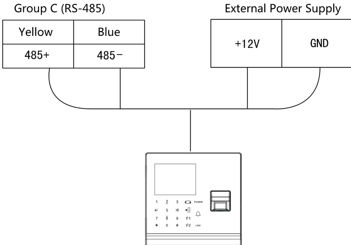
Figure 4-5 Wiring of RS-485 Output
