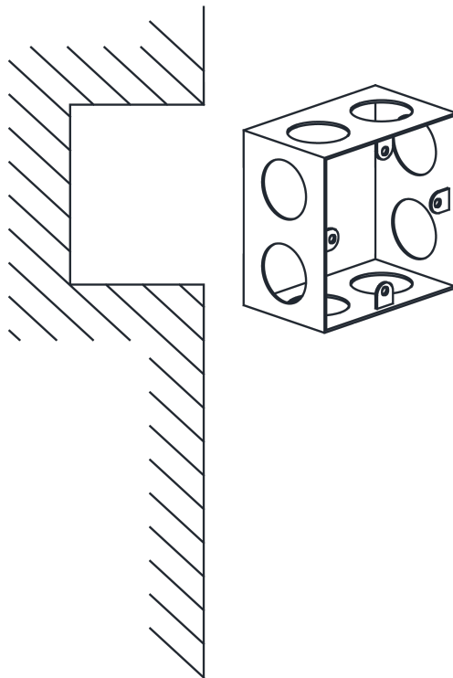
Figure 3-1 Install 86 Gang box
