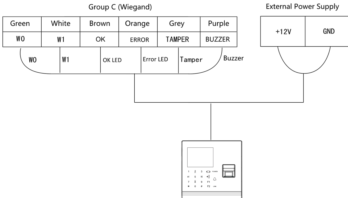
Figure 4-6 Wiring as Wiegand Card Reader
