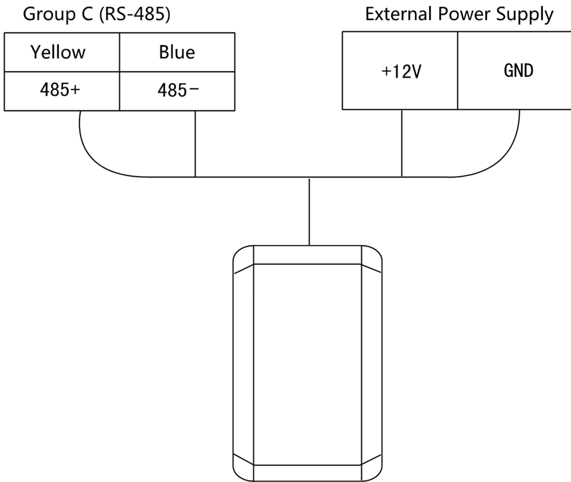
Figure 4-3 Wiring of External RS-485 Card Reader
