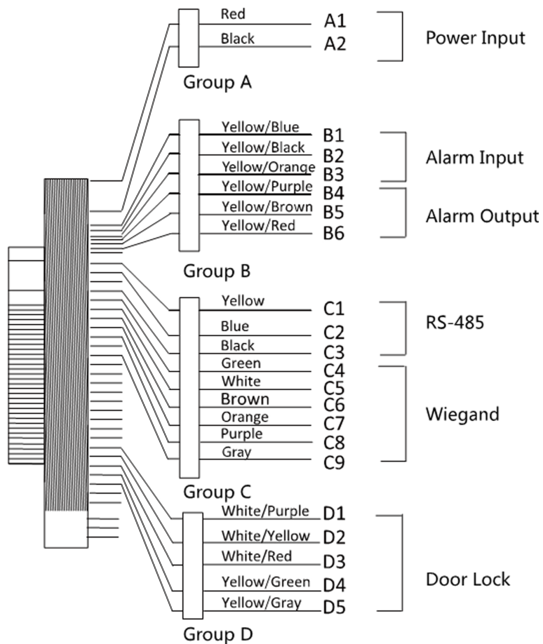
Figure 4-1 Terminal Diagram
