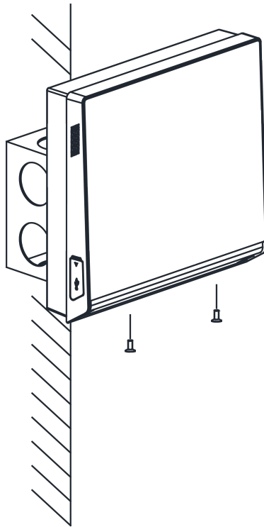
Figure 3-8 Tighten Screws
