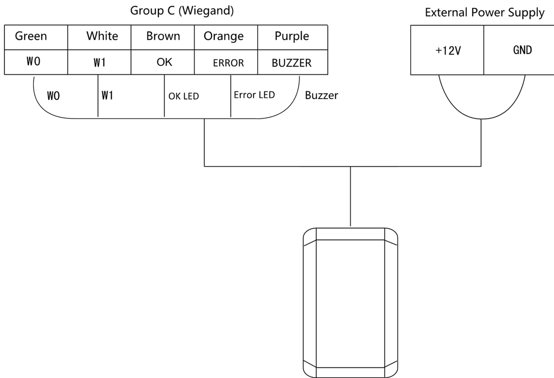
Figure 4-4 Wiring of Wiegand Card Reader
