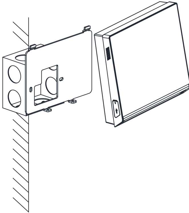
Figure 3-7 Buckle Terminal on Plate
