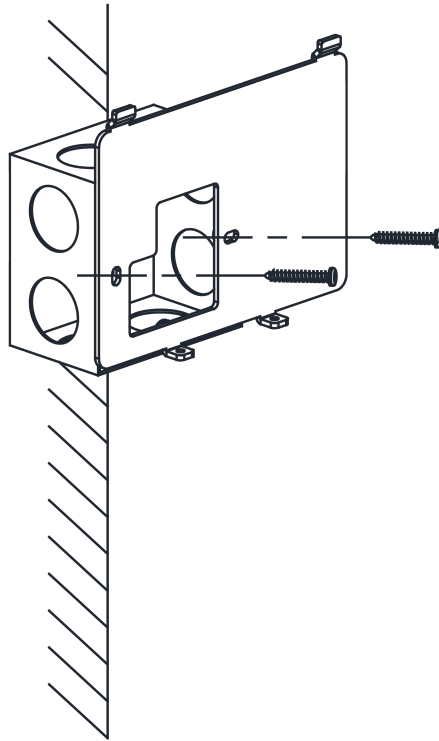
Figure 3-6 Install Mounting Plate
