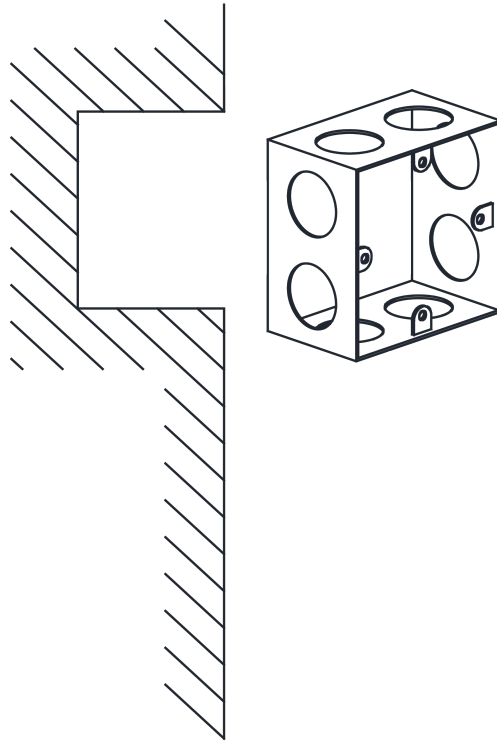
Figure 3-5 Install 86 Gang box
