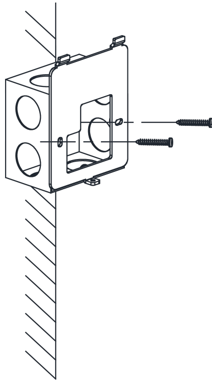
Figure 3-2 Install Mounting Plate
