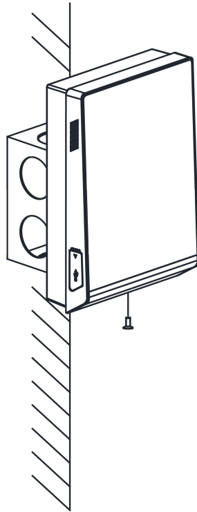
Figure 3-4 Tighten Screw
