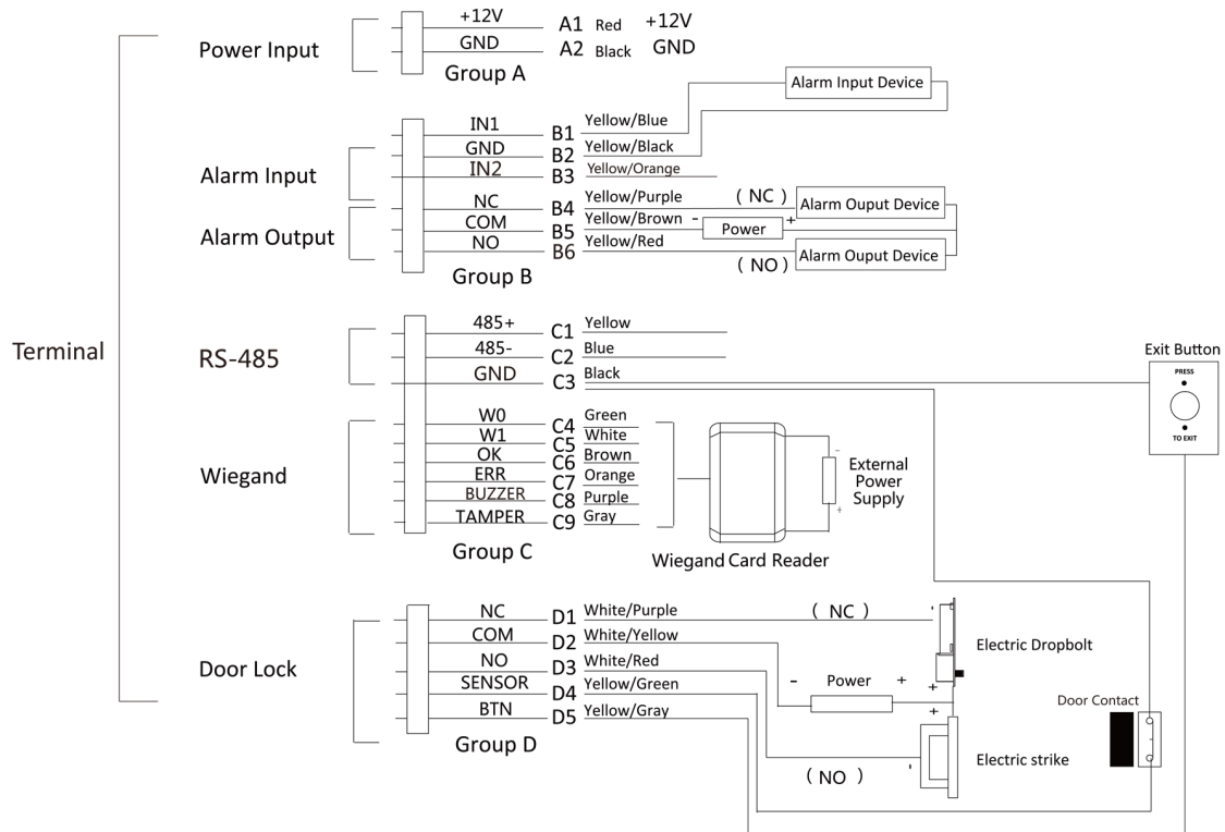
Figure 4-2 Wiring Overview
