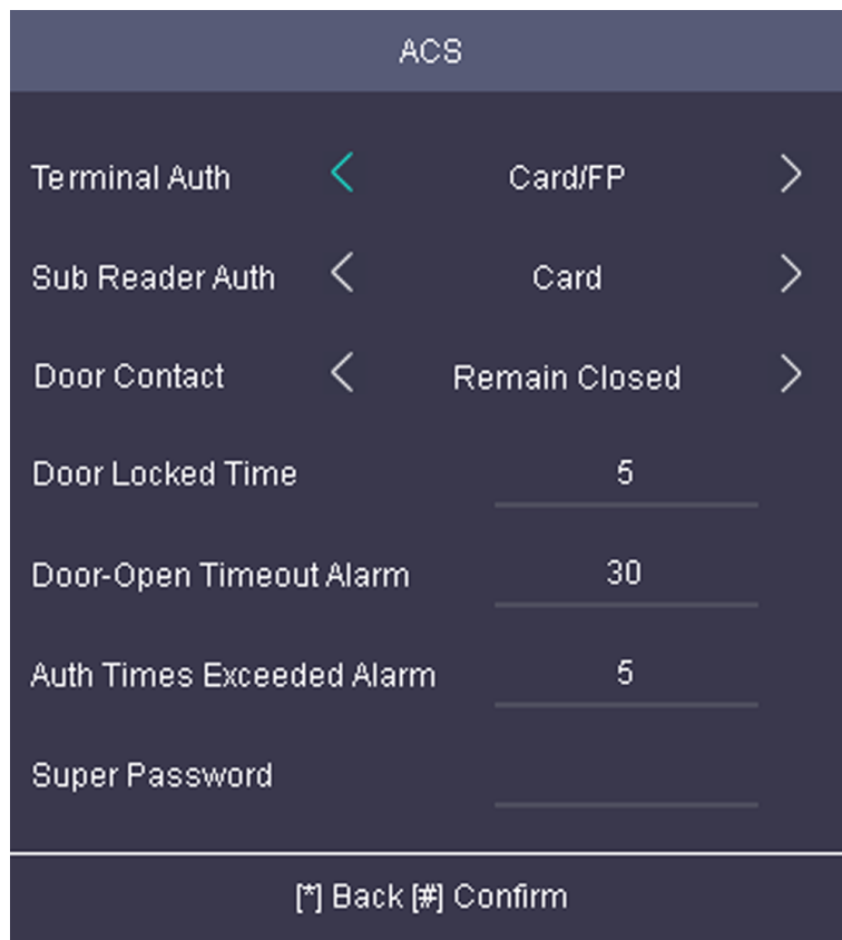
Figure 6-8 Access Control Parameters
