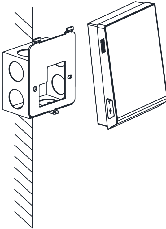
Figure 3-3 Buckle Terminal on Plate
