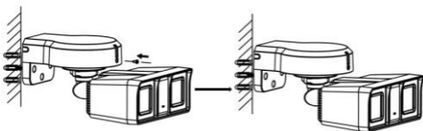
Figure 2-11 Lock Cover to Body
